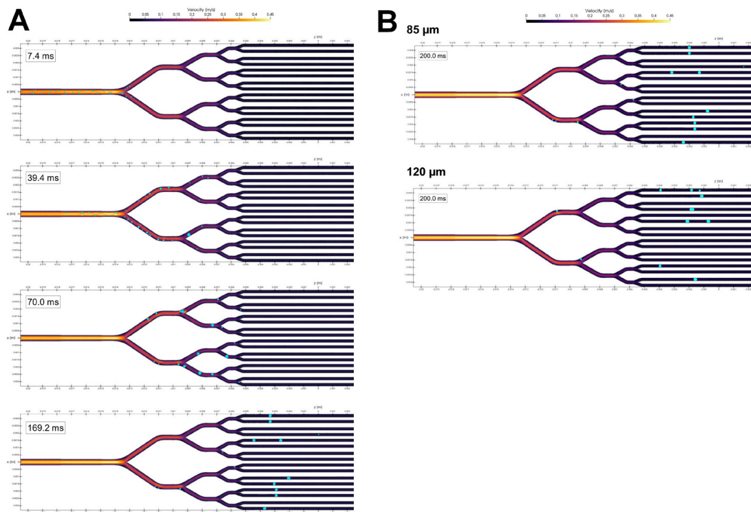
Figure 3 Illustration of the software-based simulation. (A) illustrates the vascular model and shows different points in time of the simulation using 85 µm air bubbles. At 7.4 ms the 85 µm air bubbles are not yet fused and enter the first branching. During the flow through the vascular model (39.4 ms and 70.0 ms), especially at the branchings, small bubbles fuse to larger ones, which eventually cause occlusions of the terminal vessels. A few bubbles adhere to the vessel walls within the model. (B) shows the end of simulations using 85 µm and 120 µm air bubbles. At this point, eight of the terminal vessels are occluded, while using 120 µm bubbles, occlusion in only six vessels was observed. This qualitative analysis is in line with the findings of the in vivo experiments.
