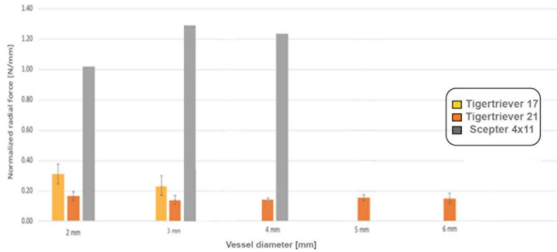
Figure 4. Comparison of the radial force of Tiger stentriever with Percutaneous transluminal angioplasty (PTA) balloons. In vitro comparison of the radial force exerted by the Tigerstentriever 17 and 21 with PTA balloons in different vessel diameters. The radial force of PTA balloons is constantly higher
