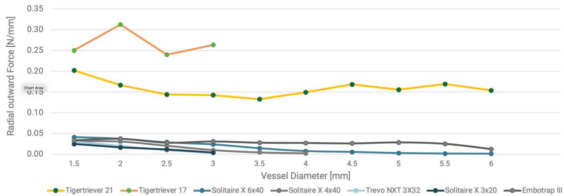
Figure 3. Comparison of the radial force of different stentriever. In vitro comparison of the radial force exerted by the Tigertrievers 21 and 17 with other commercially available stent retrievers. The Tigertriever device has a consistently higher radial force across various vessel diameters.
